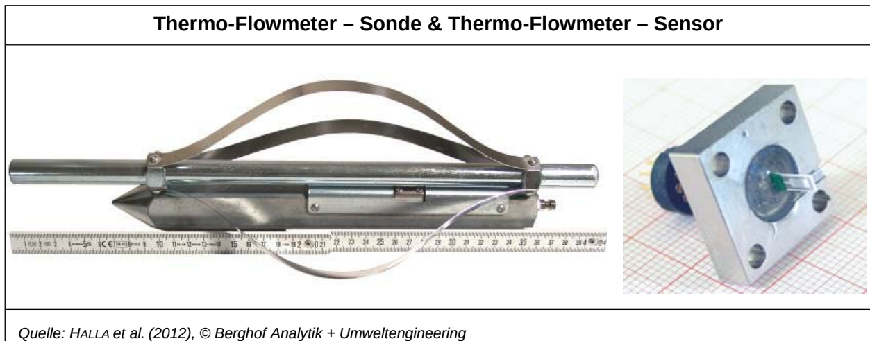
Abbildung 19: links: Thermo-Flowmeter – Sonde, rechts: Thermo-Flowmeter – Sensor.
